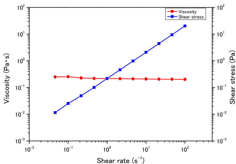
Fig. 1 Flow curves of TB3094F (at 25°C)
