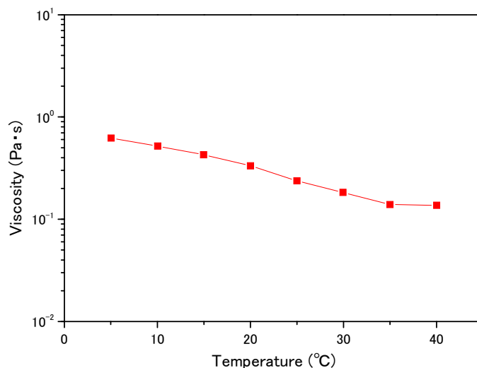
Fig. 2 Temperature-viscosity curve of TB3094F
