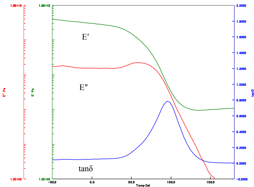
Fig. 3 Results of DMA measurement of TB3094F
