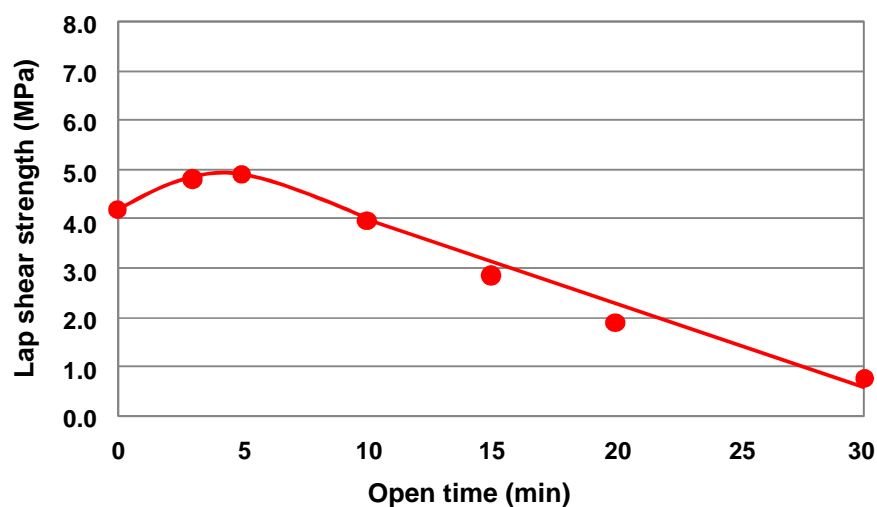
Fig. 2 Open time and lap shear strength of TB1533C Bonding after prescribed open time Curing conditions: At 23°C and 50%RH for 7 days Measuring conditions: 3TS-4100-013 Bonding of aluminum (A1050P) test pieces/Application to both surfaces/ Bonding after prescribed open time
