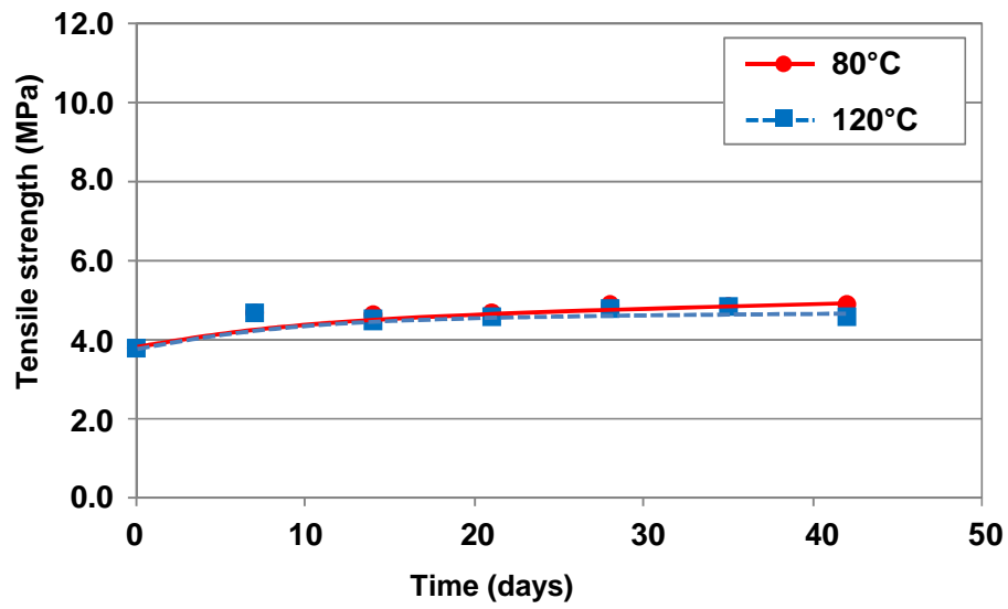
Fig. 7 Heat resistance (tensile strength) of TB1533C Curing conditions: At 23°C and 50%RH for 7 days Measuring conditions: TS-4190-001
