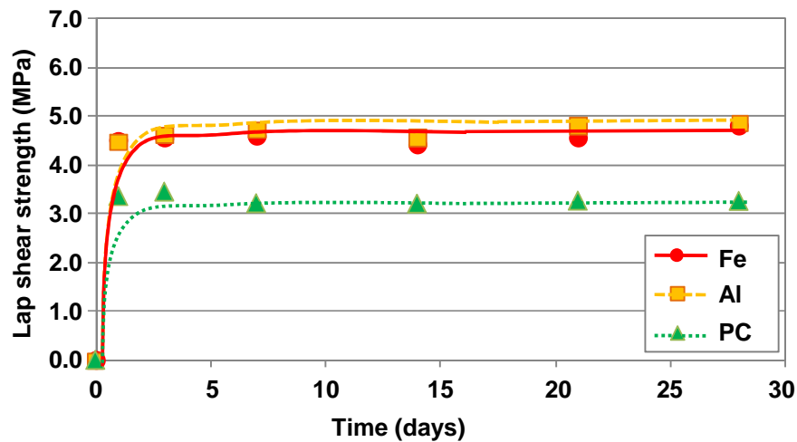
Fig. 4 Curing time and lap shear strength of TB1533C
