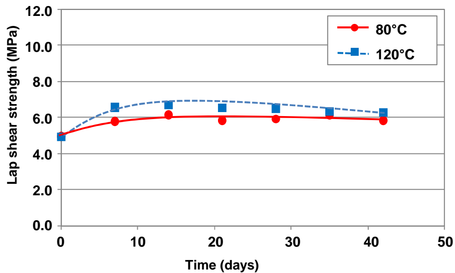
Fig. 6 Heat resistance (lap shear strength) of TB1533C
