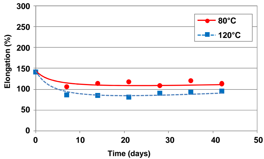
Fig. 8 Heat resistance (elongation) of TB1533C Curing conditions: At 23°C and 50%RH for 7 days Measuring conditions: 3TS-4190-001
