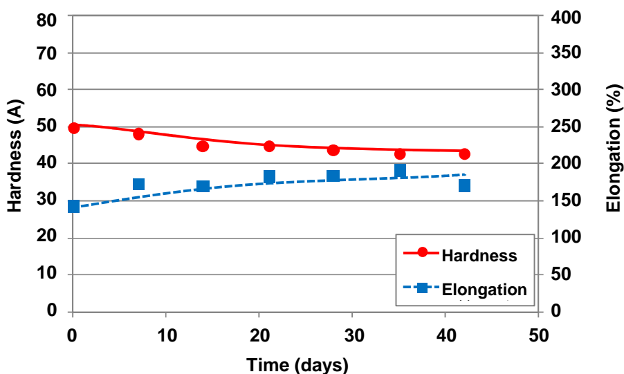
Fig. 11 Moisture resistance (hardness and elongation) of TB1533C Curing conditions: At 23°C and 50%RH for 7 days Environmental conditions: 85°C, 85%RH Measuring conditions: 3TS-2B00-004, 3TS-4190-001
