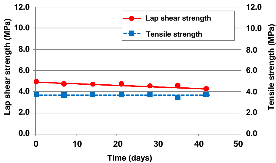
Fig. 10 Moisture resistance (lap shear strength and tensile strength) of TB1533C Curing conditions: At 23°C and 50%RH for 7 days Environmental conditions: 85°C, 85%RH Measuring conditions: 3TS-4190-001, 3TS-4100-013 Bonding of aluminum (A1050P) test pieces/Application to both surfaces/ Bonding after 5-minute open time
