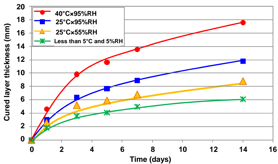
Fig. 1 Curing ability of TB1533C depending on temperature and relative humidity Measuring conditions: 3TS-3160-005
