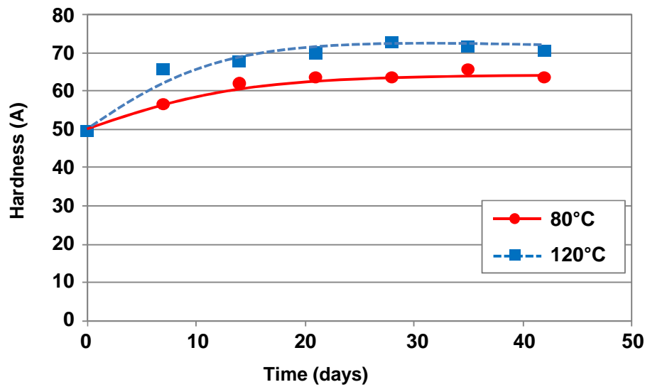
Fig. 9 Heat resistance (hardness) of TB1533C Curing conditions: At 23°C and 50%RH for 7 days Measuring conditions: 3TS-2B00-004
