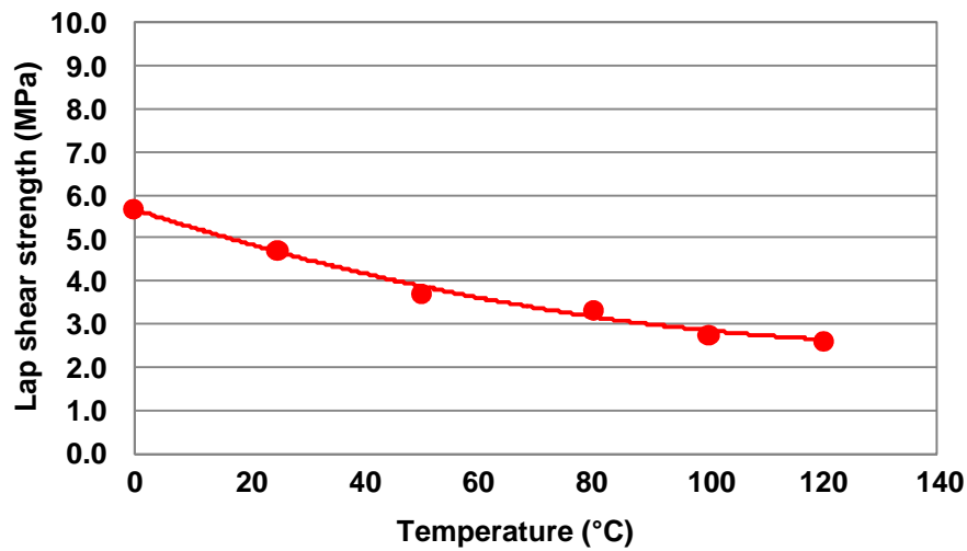
Fig. 3 Lap shear strength of TB1533C when heated
