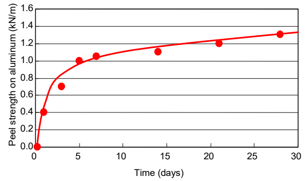
Fig. 7 Dependence of peel strength of TB1537D on curing time
