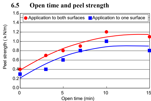
Fig. 6 Dependence of peel strength of TB1537D on open time and application condition (one or both surfaces)
