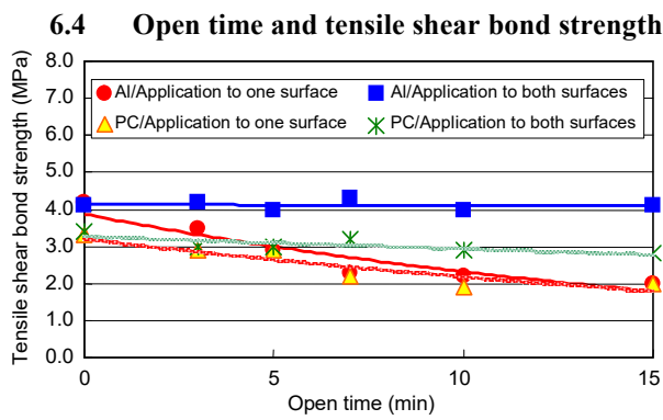
Fig. 5 Dependence of tensile shear bond strength of TB1537D on open time and application condition (one or both surfaces)
