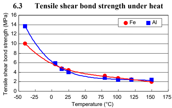
Fig. 4 Tensile shear bond strength of TB1537D under heat
