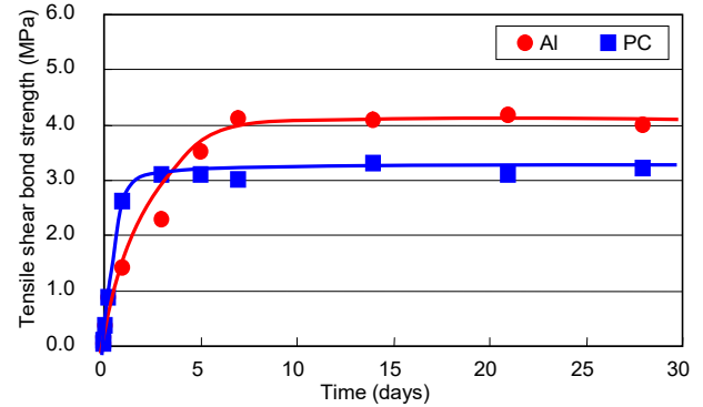
Fig. 8 Dependence of tensile shear bond strength of TB1537D on curing time
