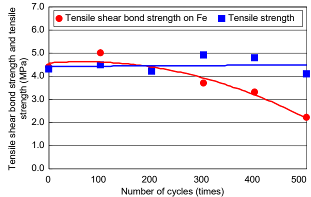
Fig. 9 Dependence of bonding strength of TB1537D on number of heat cycles
