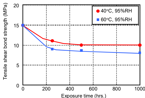
Fig. 3 Moisture resistance of TB7781
