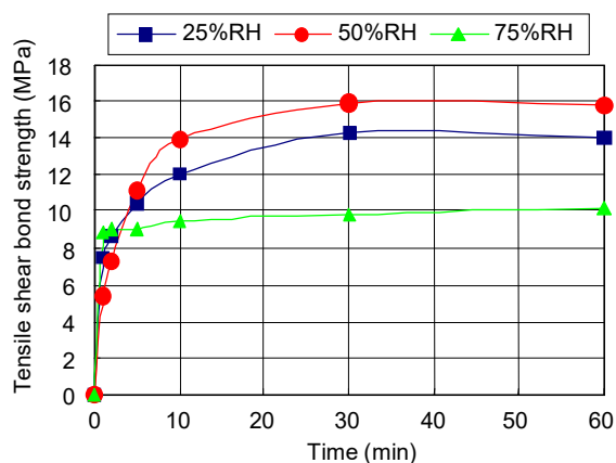
Fig. 1 Adhesion of TB7781 under various humidity conditions
