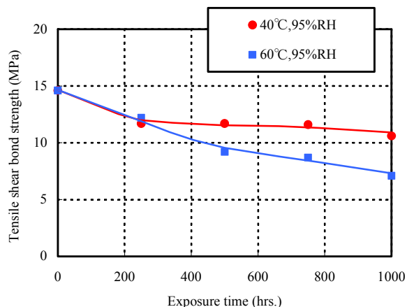
Fig. 3 Moisture resistance of TB7785
