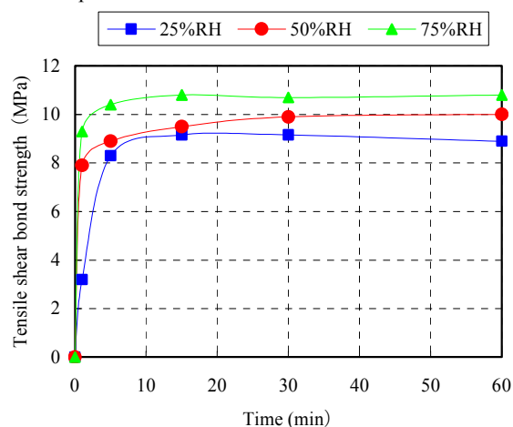
Fig. 1 Adhesion of TB7785 under various humidity conditions
