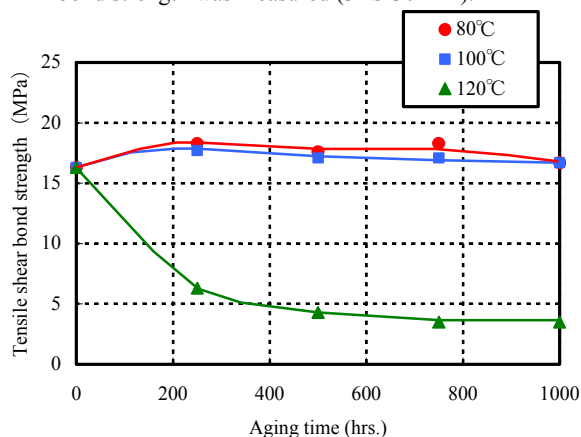
Fig. 2 Thermal resistance of TB7785
